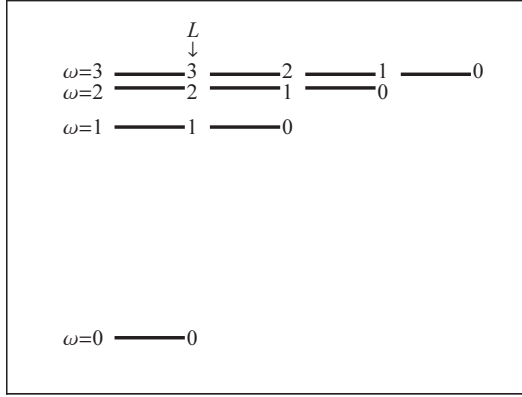
Fig. 12.3. The spectrum of the three-dimensional Coulomb problem. States up to \omega = 3 are shown. The principal quantum number is n = \omega + 1
