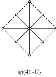
Fig. 2.3. Root diagram of the algebra C_2
