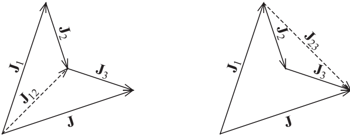
Fig. 6.1. Coupling schemes of three angular momentum vectors, \mathbf{J}_1 , \mathbf{J}_2 , and \mathbf{J}_3
