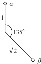
Fig. 2.7. Simple roots of B_2
